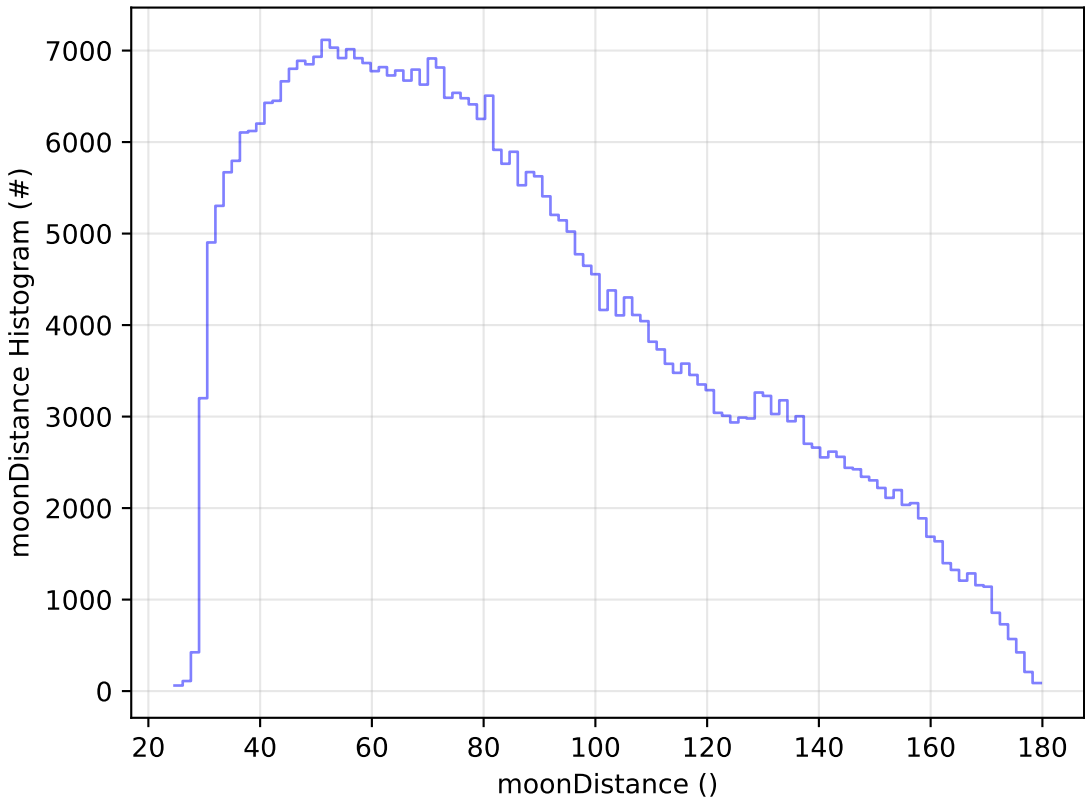
start_date_do-270v3.4_10yrs WFD z band: moonDistance Histogram
