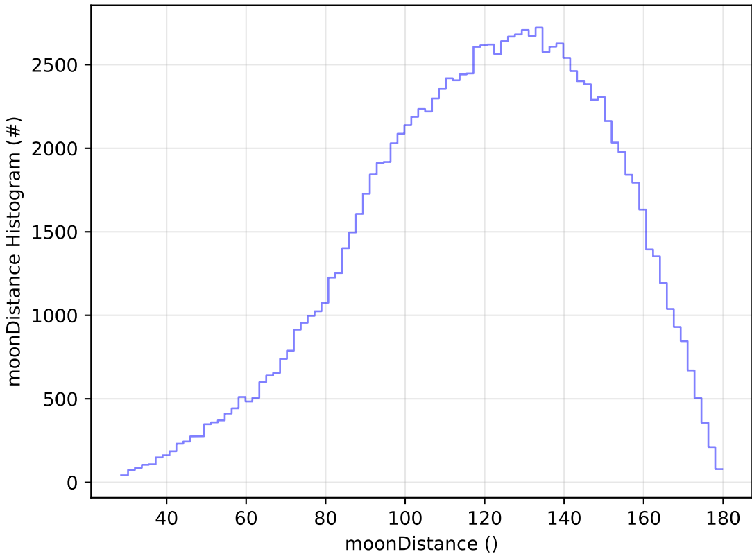
start_date_do-270v3.4_10yrs WFD u band: moonDistance Histogram
