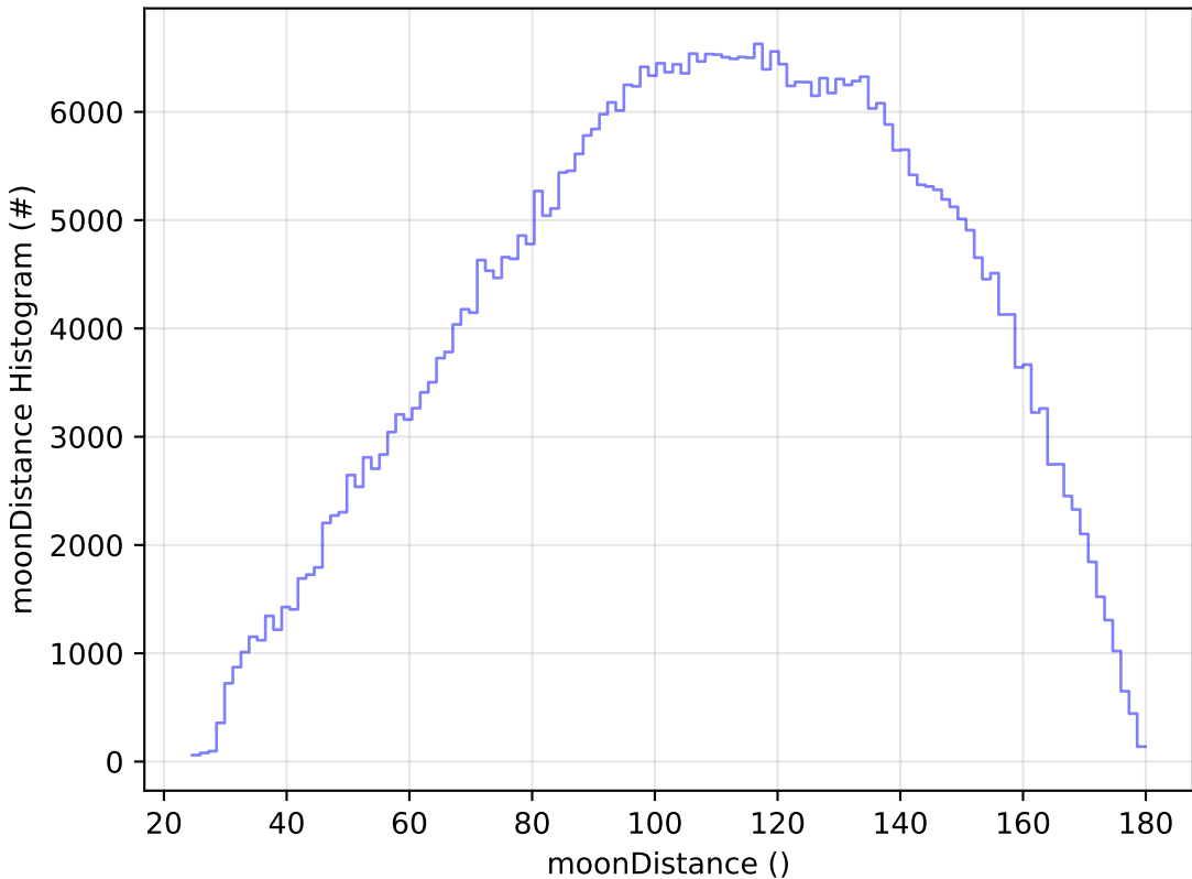
start_date_do-270v3.4_10yrs WFD r band: moonDistance Histogram
