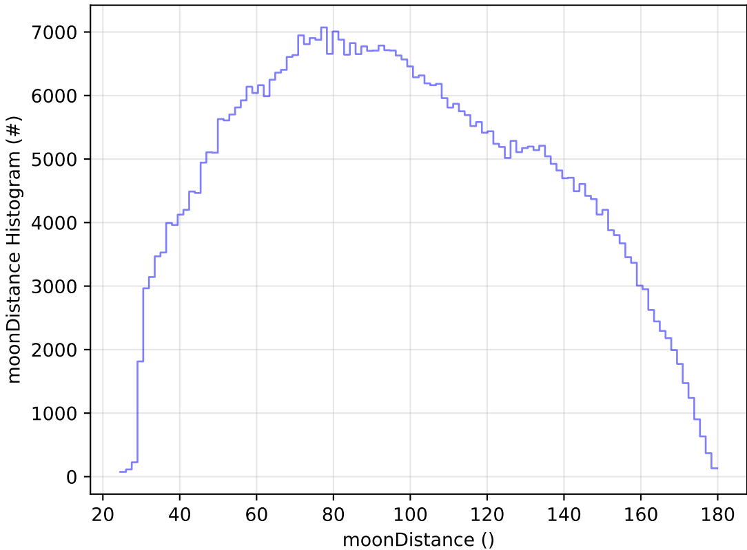
start_date_do-270v3.4_10yrs WFD i band: moonDistance Histogram
