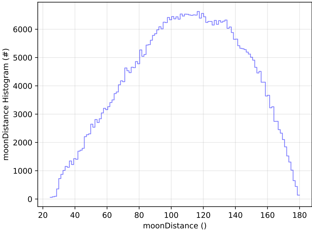
start_date_do-270v3.4_10yrs All sky r band: moonDistance Histogram
