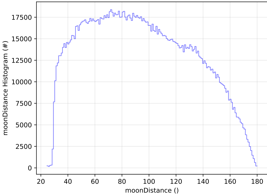
start_date_do-270v3.4_10yrs All sky all bands: moonDistance Histogram
