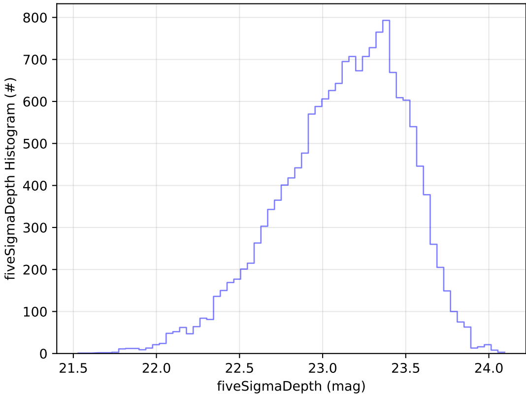
start_date_do-270v3.4_10yrs Yr 1 u band: fiveSigmaDepth Histogram
