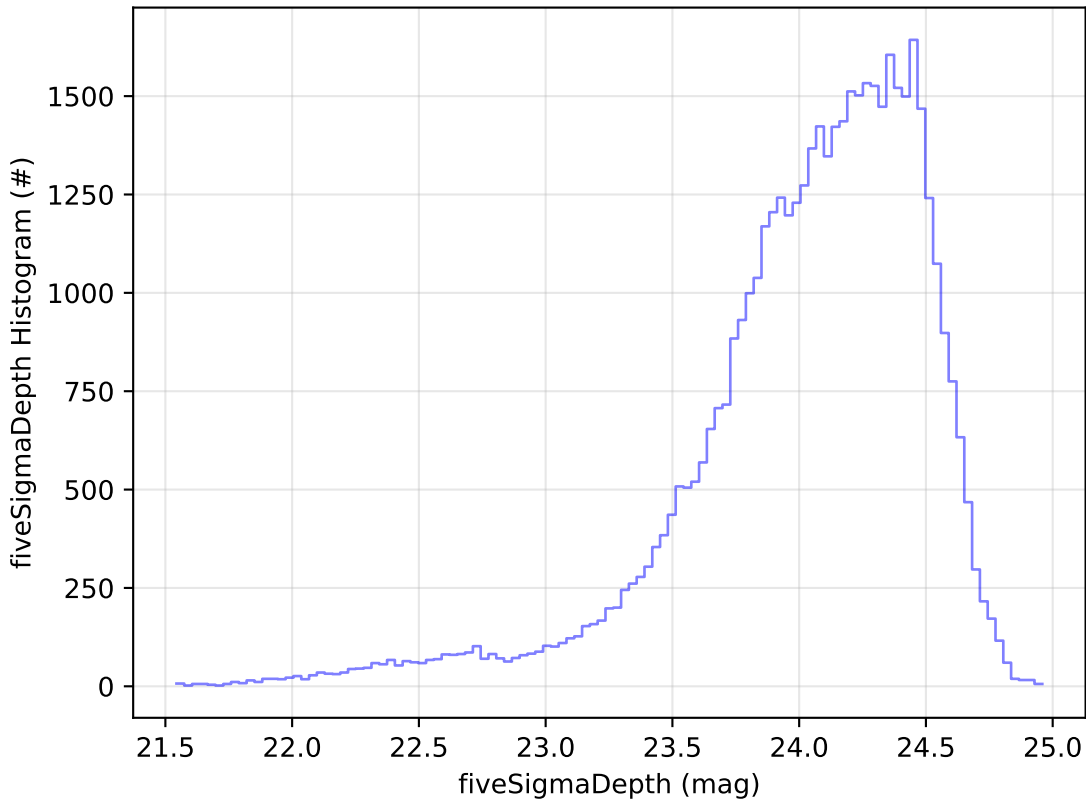
start_date_do-270v3.4_10yrs Yr 1 r band: fiveSigmaDepth Histogram
