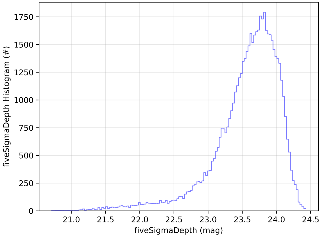
start_date_do-270v3.4_10yrs Yr 1 i band: fiveSigmaDepth Histogram
