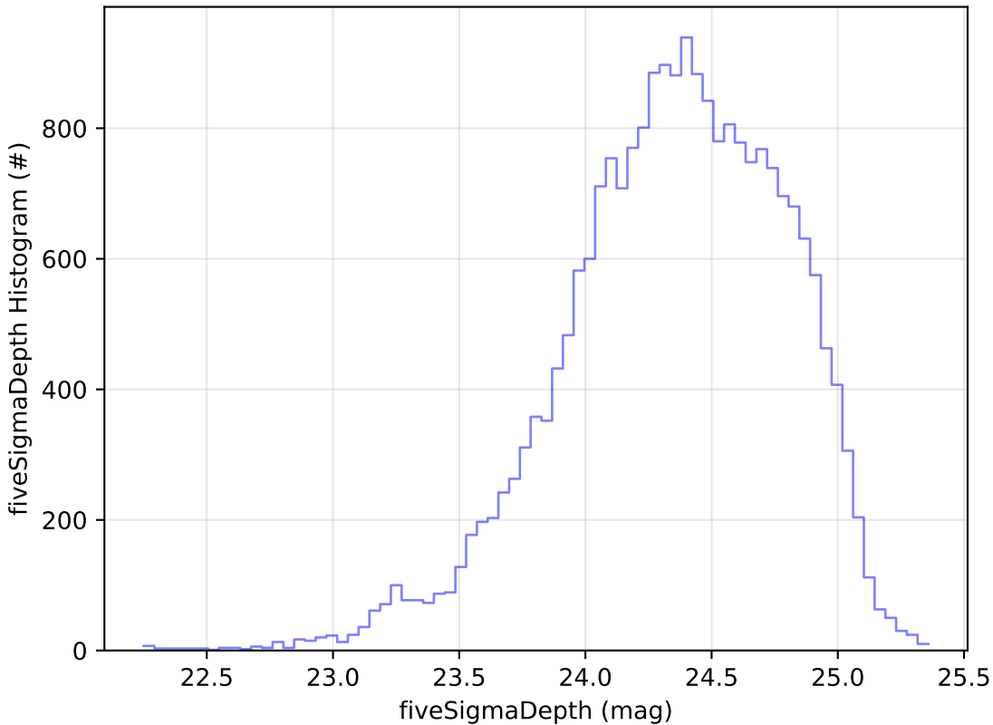
start_date_do-270v3.4_10yrs Yr 1 g band: fiveSigmaDepth Histogram
