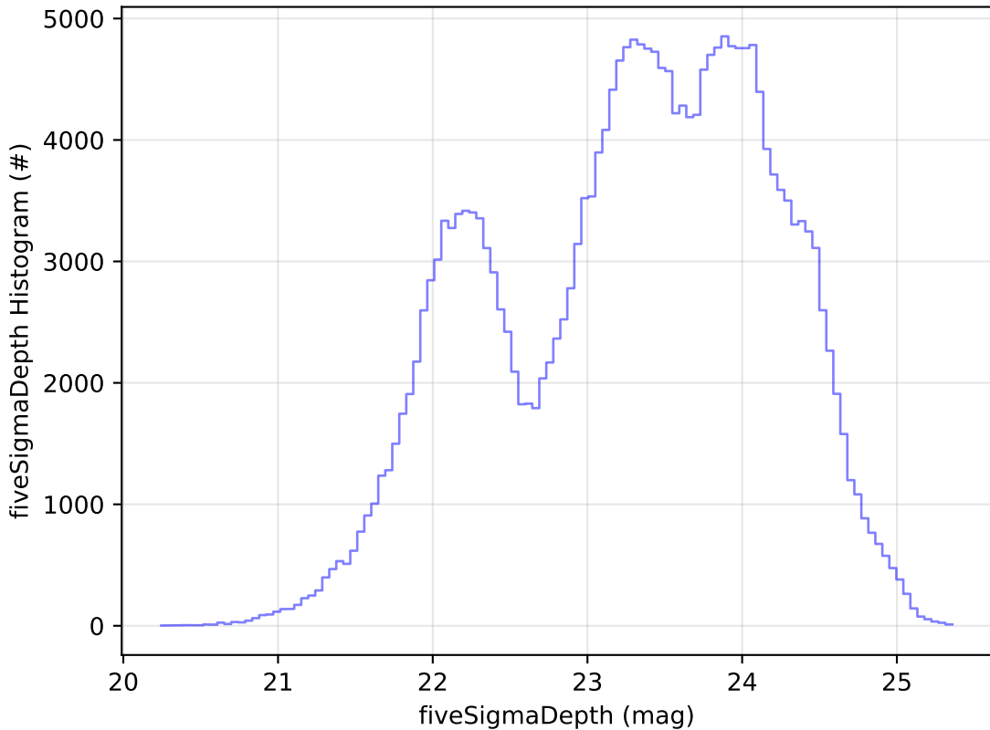
start_date_do-270v3.4_10yrs Yr 1 all bands: fiveSigmaDepth Histogram
