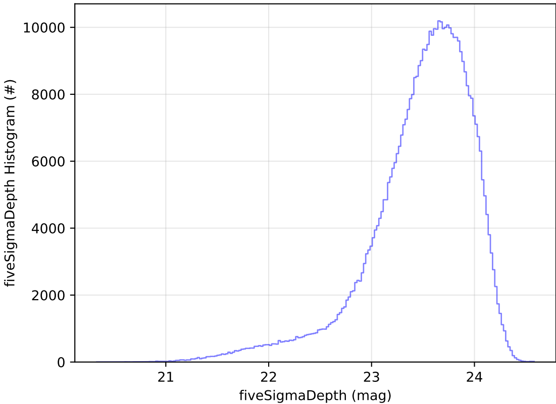
start_date_do-270v3.4_10yrs WFD i band: fiveSigmaDepth Histogram
