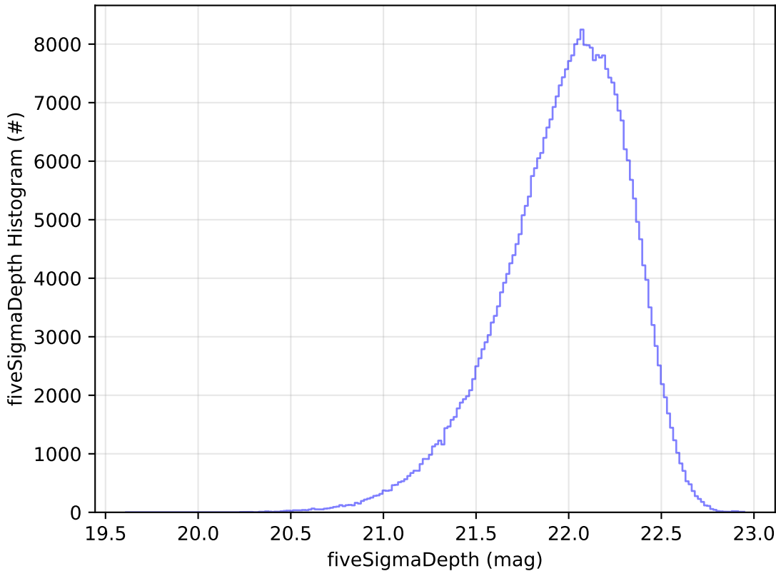
start_date_do-270v3.4_10yrs All sky y band: fiveSigmaDepth Histogram
