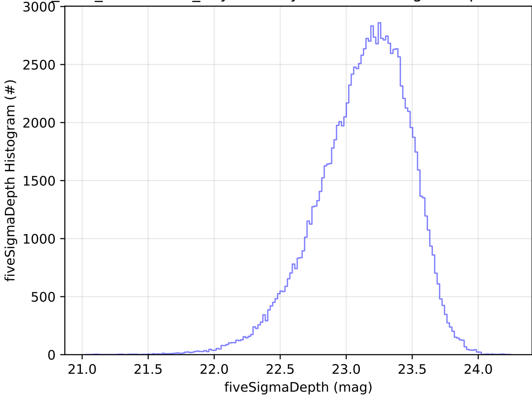
start_date_do-270v3.4_10yrs All sky u band: fiveSigmaDepth Histogram
