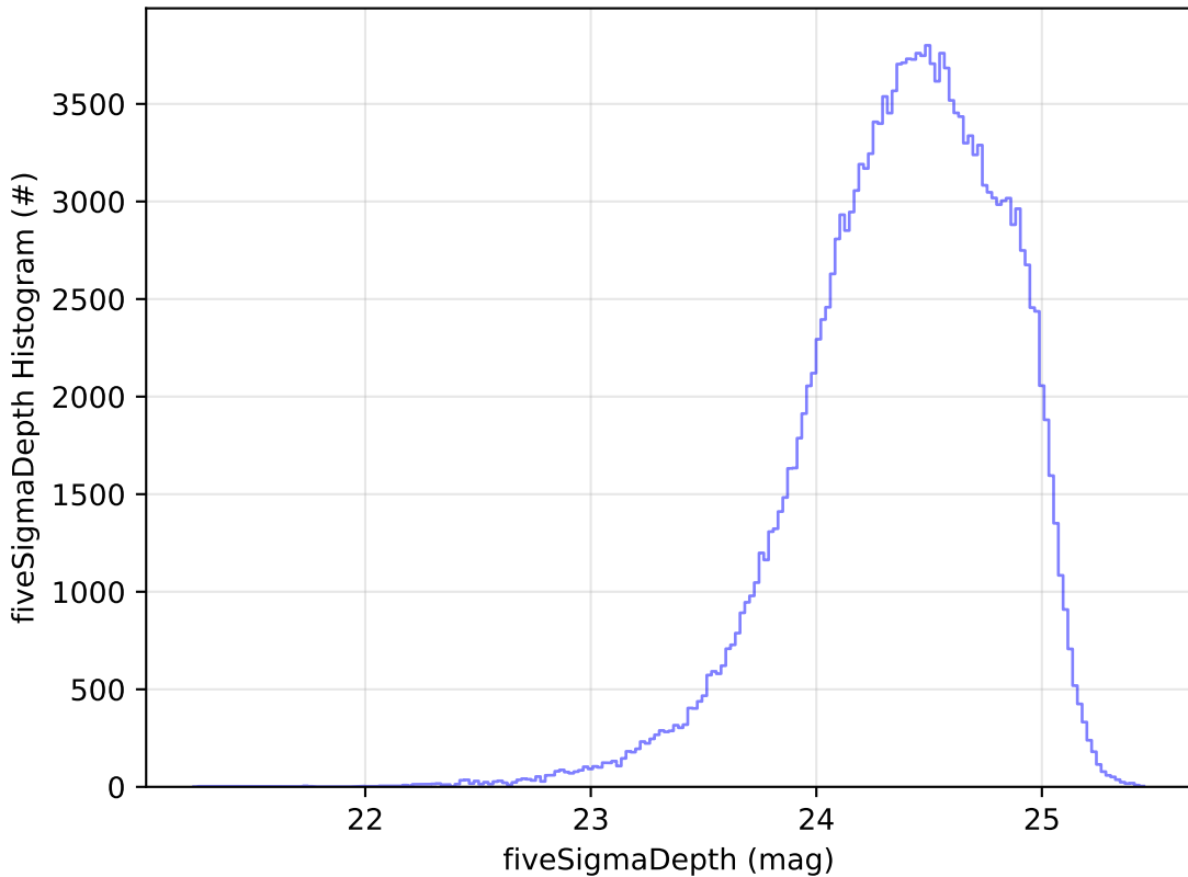
start_date_do-270v3.4_10yrs All sky g band: fiveSigmaDepth Histogram
