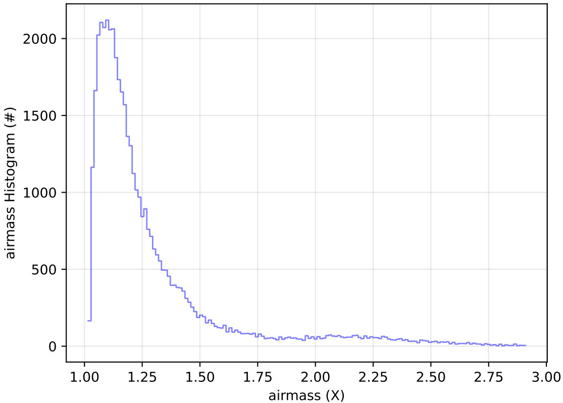
start_date_do-270v3.4_10yrs Yr 1 z band: airmass Histogram
