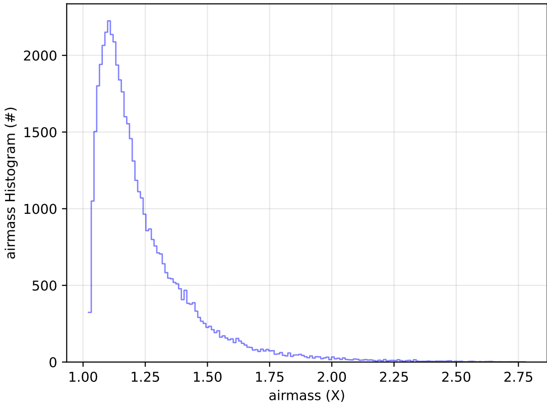
start_date_do-270v3.4_10yrs Yr 1 y band: airmass Histogram
