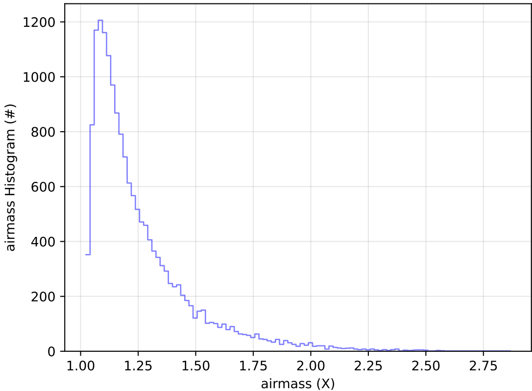
start_date_do-270v3.4_10yrs Yr 1 u band: airmass Histogram
