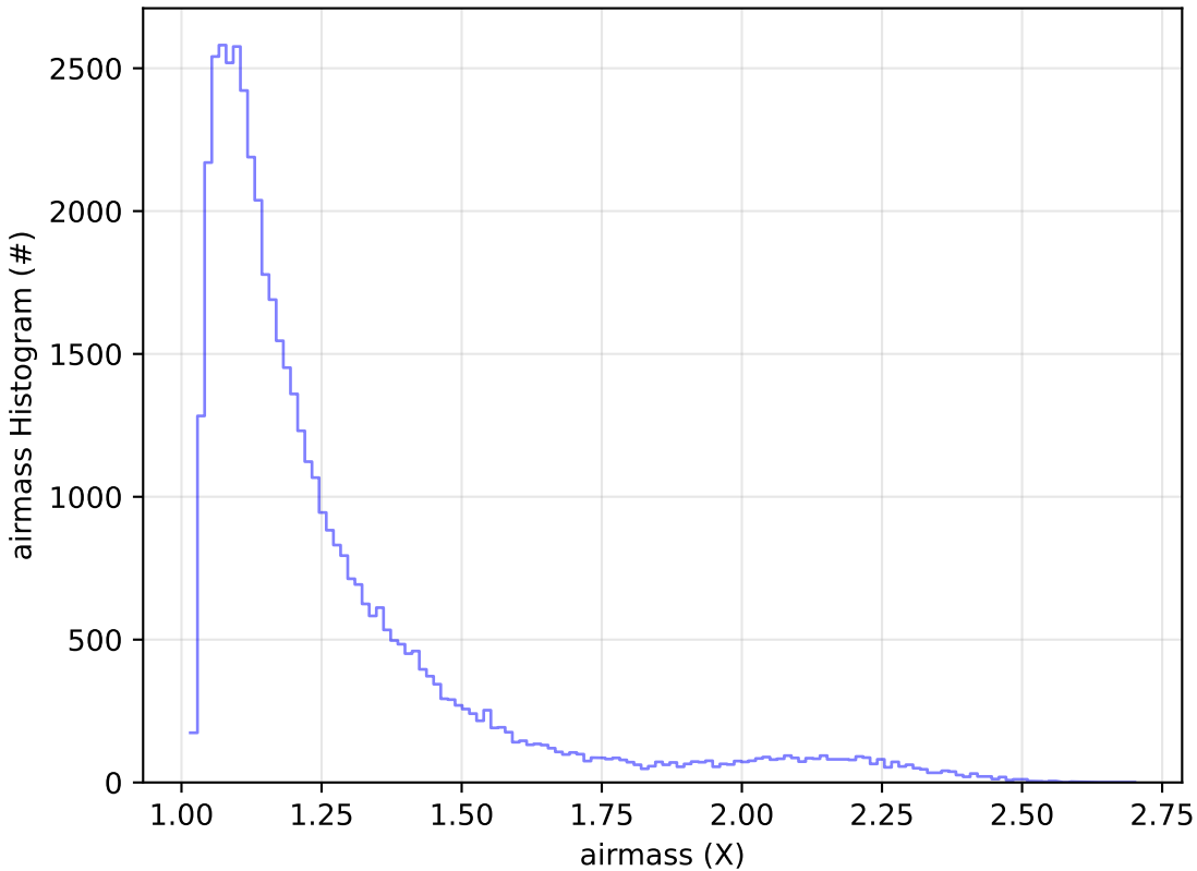
start_date_do-270v3.4_10yrs Yr 1 r band: airmass Histogram
