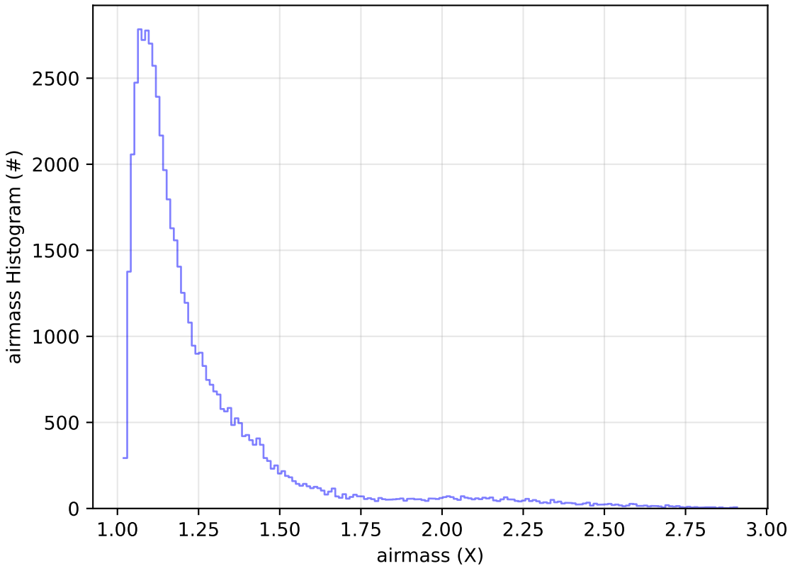
start_date_do-270v3.4_10yrs Yr 1 i band: airmass Histogram
