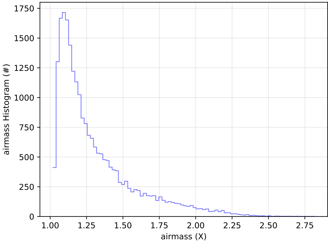
start_date_do-270v3.4_10yrs Yr 1 g band: airmass Histogram
