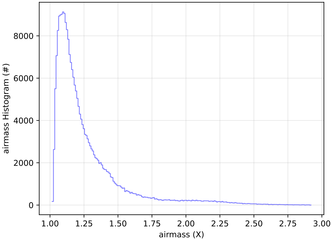
start_date_do-270v3.4_10yrs Yr 1 all bands: airmass Histogram
