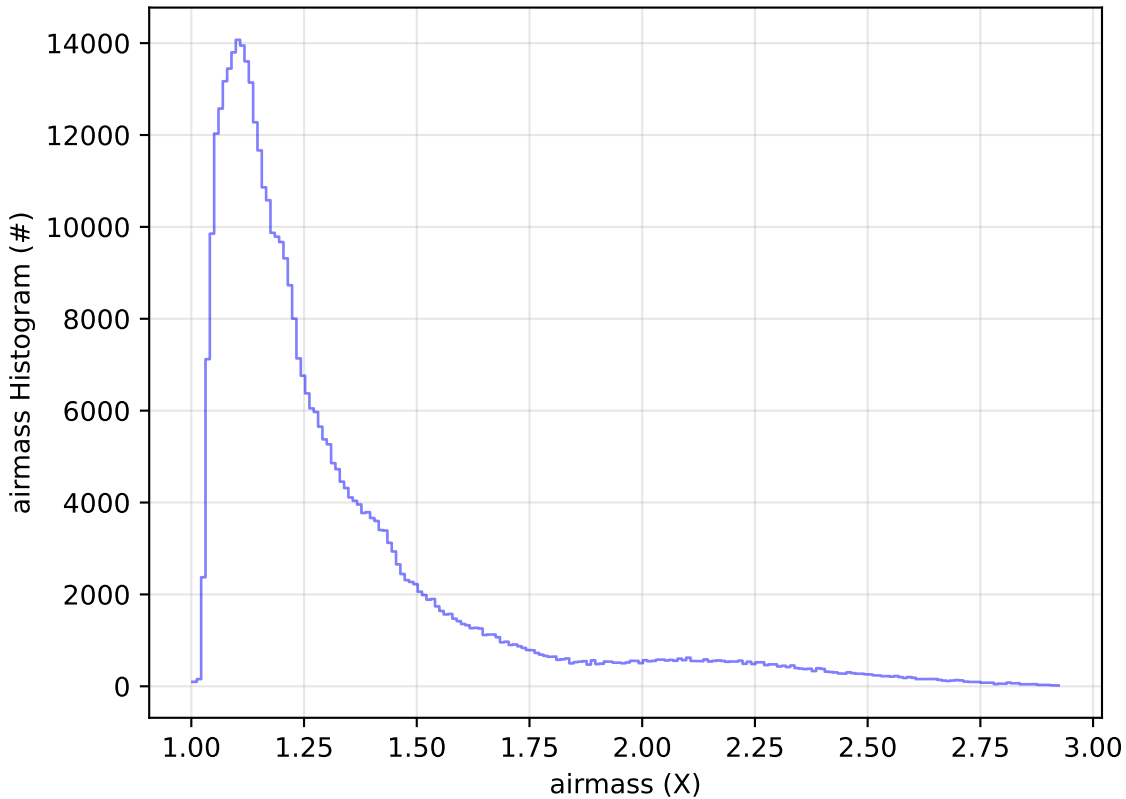
start_date_do-270v3.4_10yrs WFD z band: airmass Histogram
