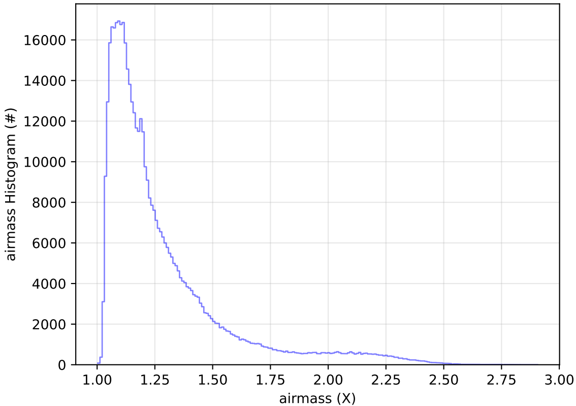
start_date_do-270v3.4_10yrs WFD r band: airmass Histogram
