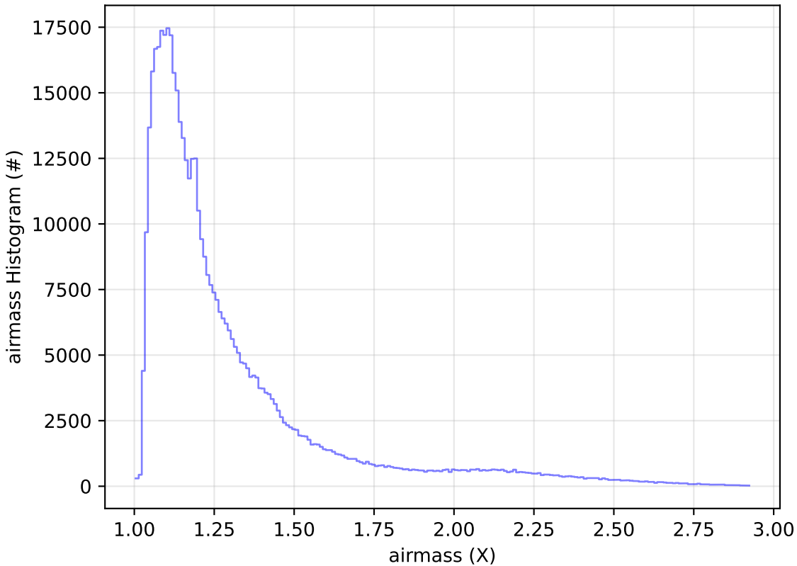
start_date_do-270v3.4_10yrs WFD i band: airmass Histogram
