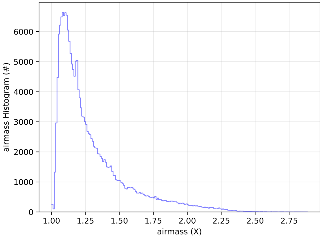
start_date_do-270v3.4_10yrs WFD g band: airmass Histogram
