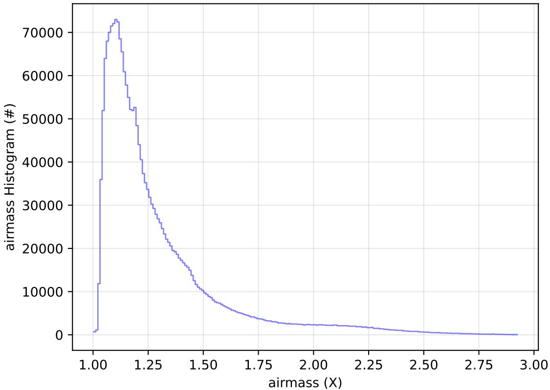
start_date_do-270v3.4_10yrs WFD all bands: airmass Histogram
