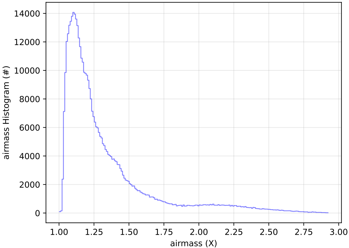
start_date_do-270v3.4_10yrs All sky z band: airmass Histogram
