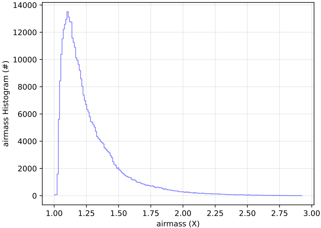
start_date_do-270v3.4_10yrs All sky y band: airmass Histogram
