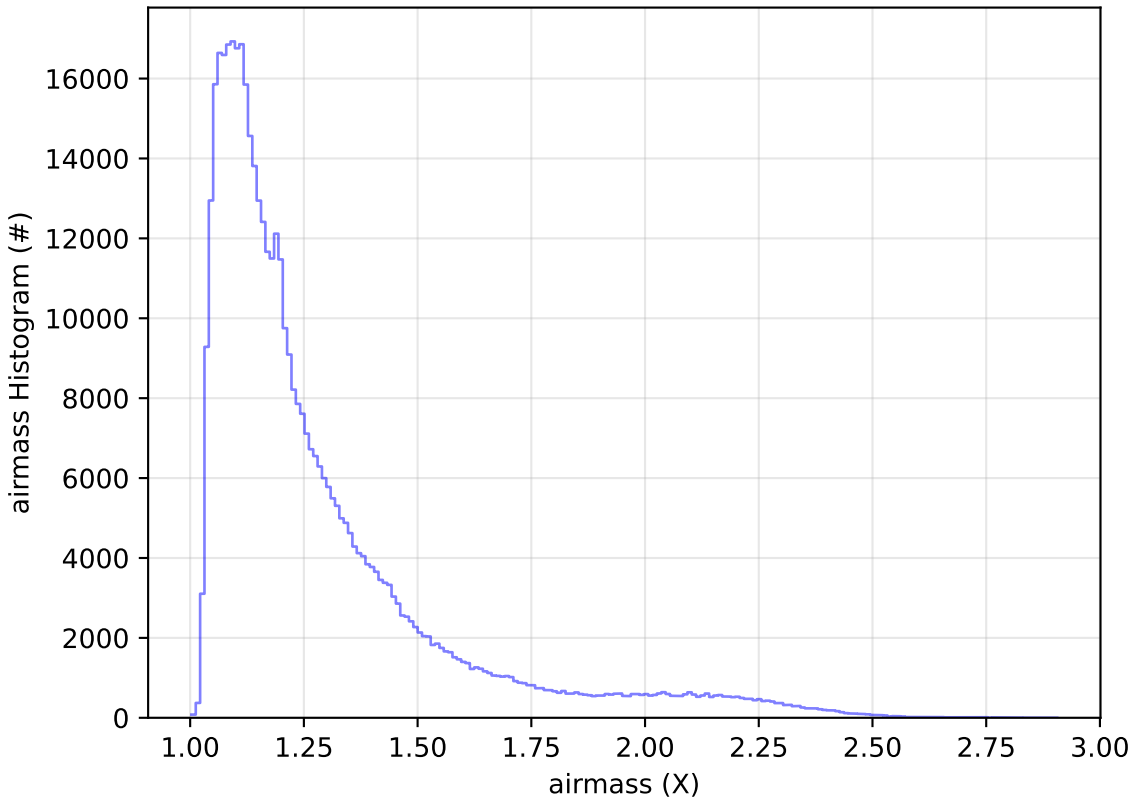
start_date_do-270v3.4_10yrs All sky r band: airmass Histogram
