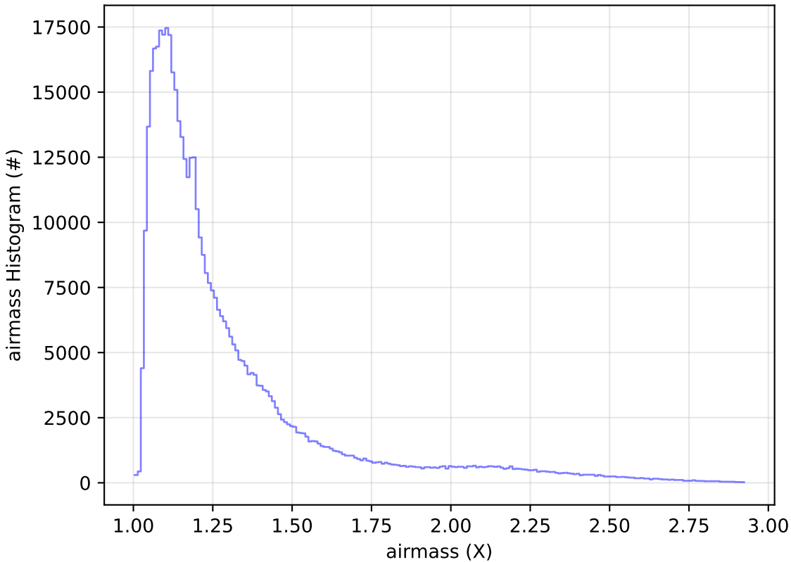
start_date_do-270v3.4_10yrs All sky i band: airmass Histogram
