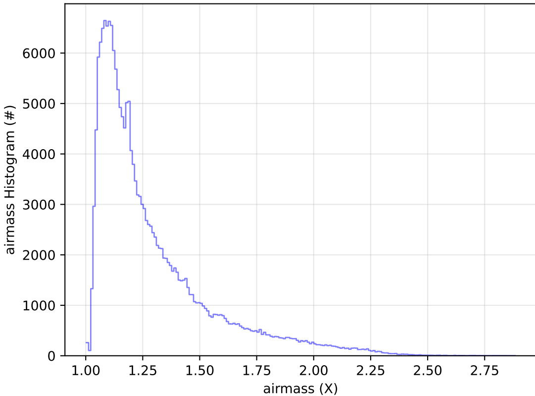
start_date_do-270v3.4_10yrs All sky g band: airmass Histogram
