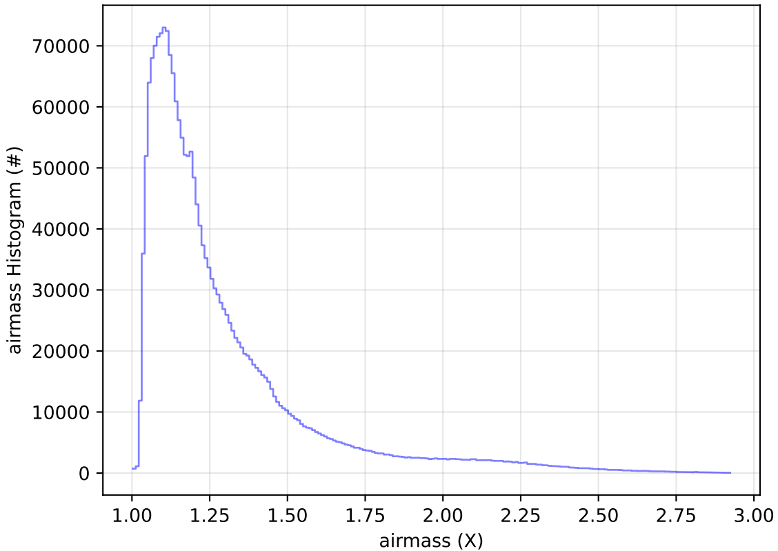
start_date_do-270v3.4_10yrs All sky all bands: airmass Histogram
