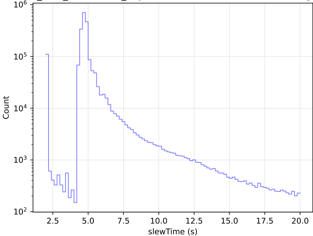
start_date_do-270v3.4_10yrs All visits: Zoom Slew Time Histogram
