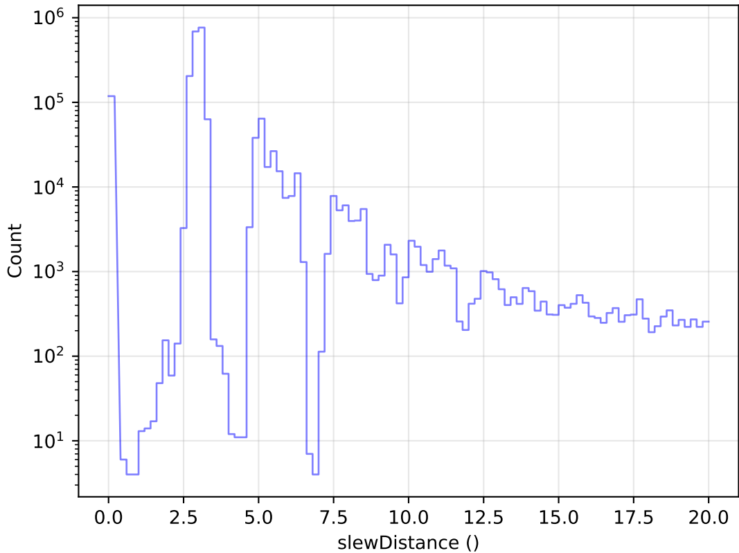
start_date_do-270v3.4_10yrs All visits: Zoom Slew Distance Histogram
