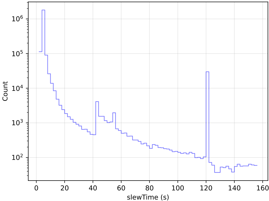
start_date_do-270v3.4_10yrs All visits: Slew Time Histogram
