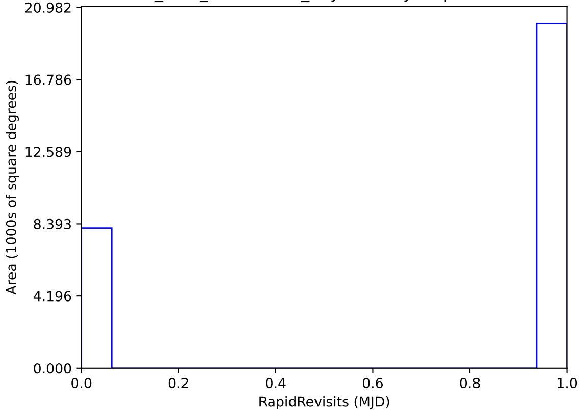
start_date_do-270v3.4_10yrs All sky: RapidRevisits
