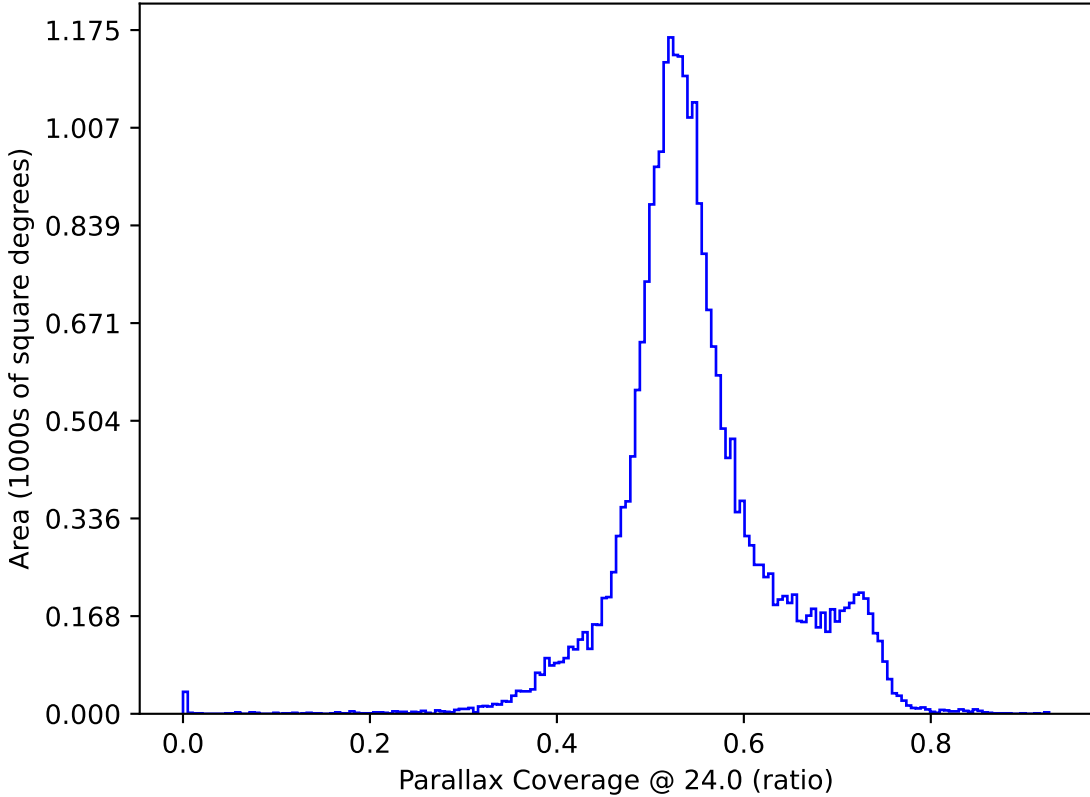
start_date_do-270v3.4_10yrs All sky: Parallax Coverage @ 24.0
