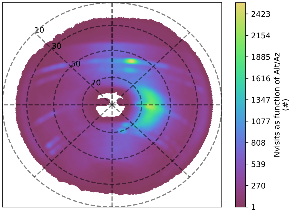
start_date_do-270v3.4_10yrs z band: Nvisits as function of Alt/Az
