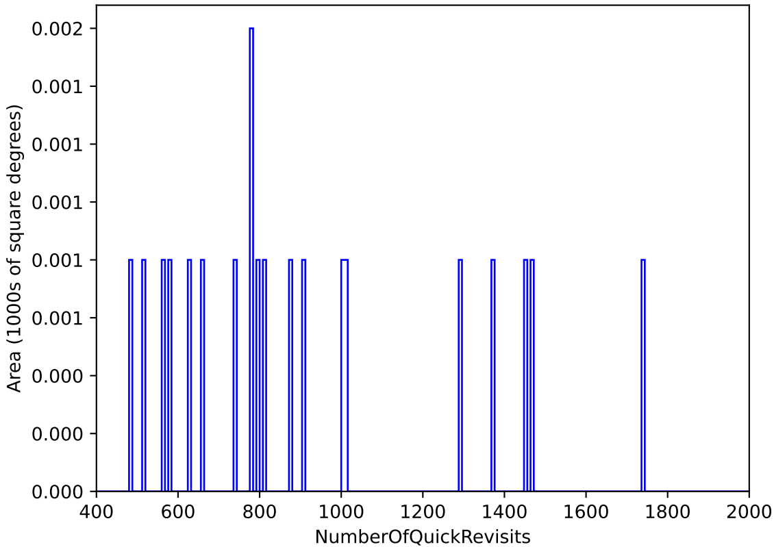
start_date_do-270v3.4_10yrs WFD: NumberOfQuickRevisits
