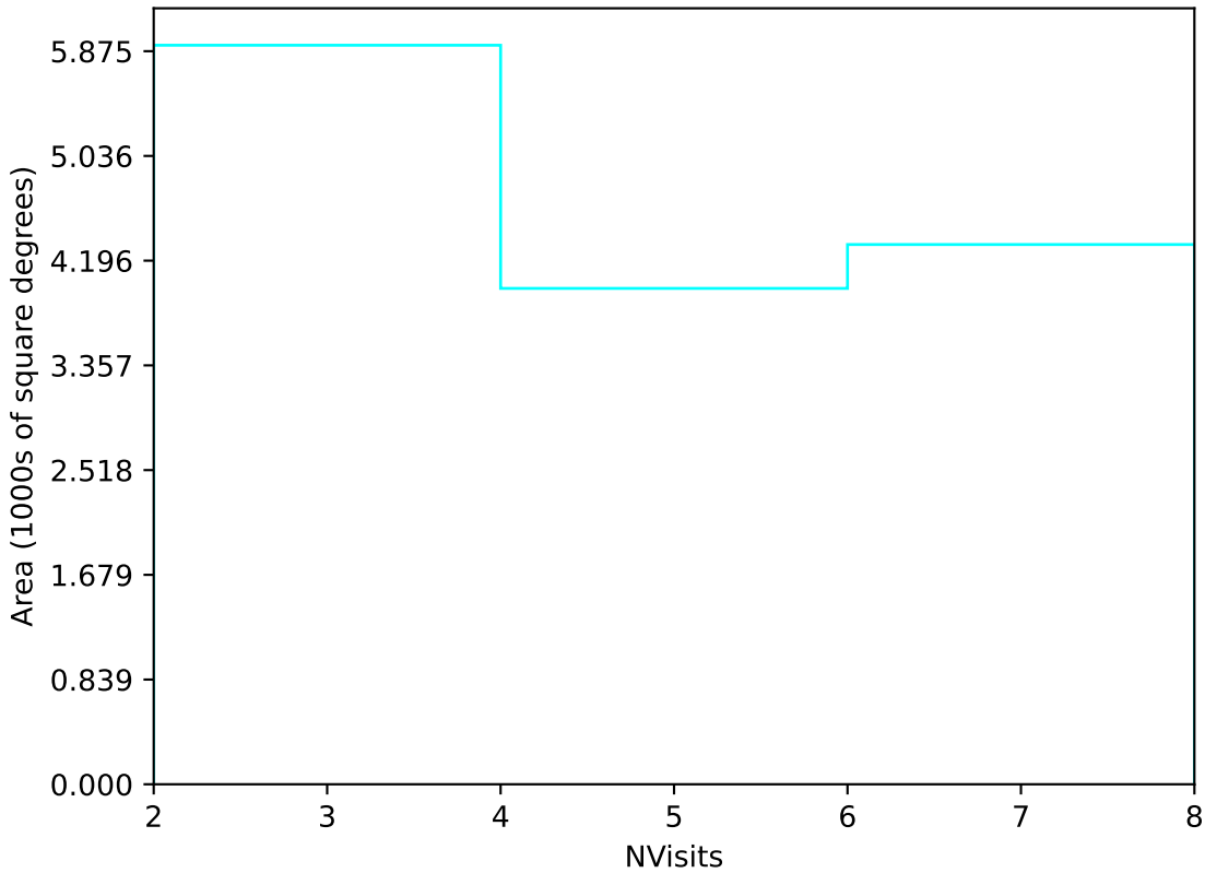
start_date_do-270v3.4_10yrs Yr 3-4 u band: NVisits
