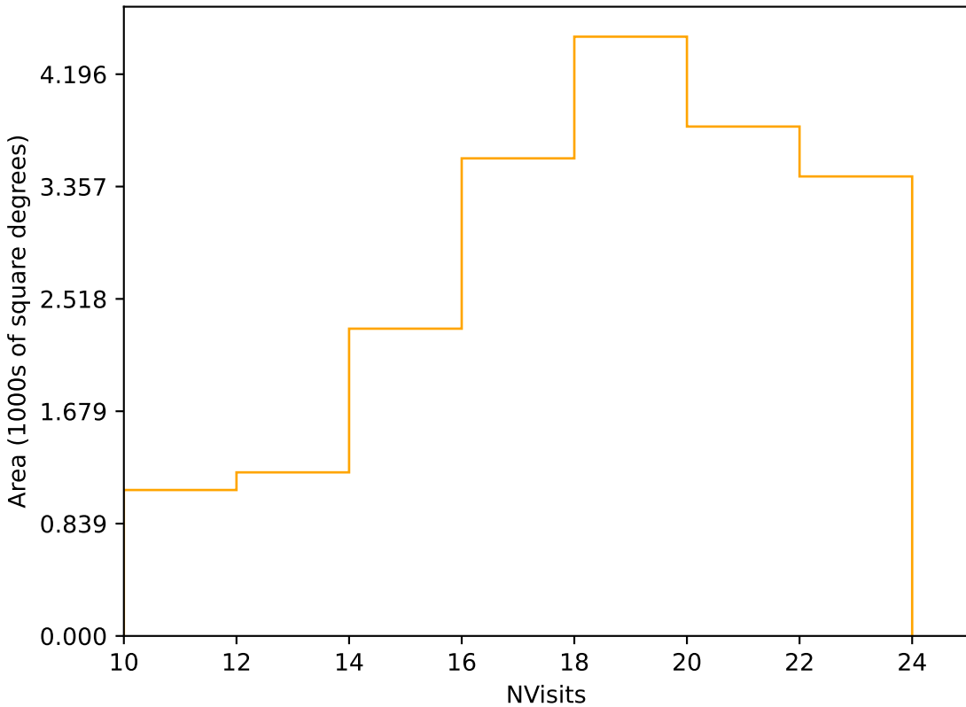
start_date_do-270v3.4_10yrs Yr 1 r band: NVisits
