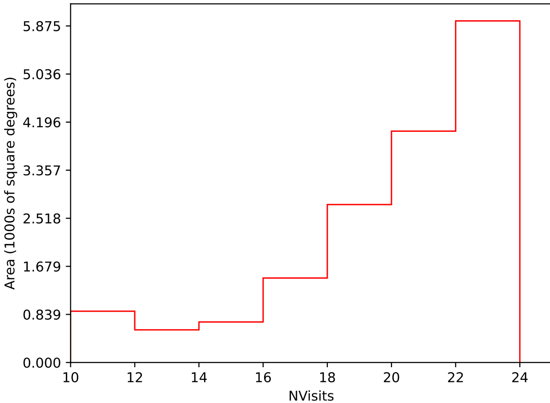
start_date_do-270v3.4_10yrs Yr 1 i band: NVisits
