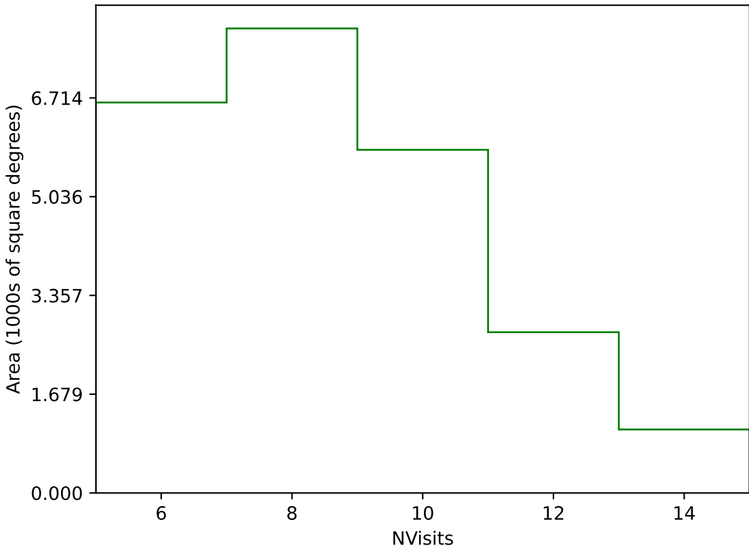
start_date_do-270v3.4_10yrs Yr 1 g band: NVisits
