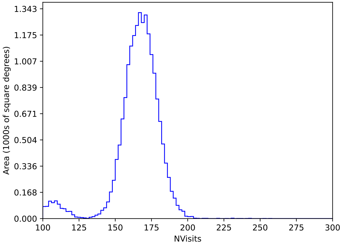
start_date_do-270v3.4_10yrs WFD y band: NVisits
