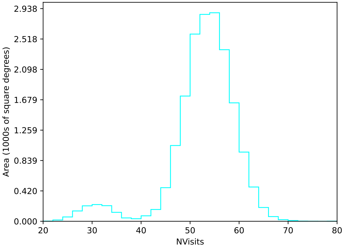
start_date_do-270v3.4_10yrs WFD u band: NVisits
