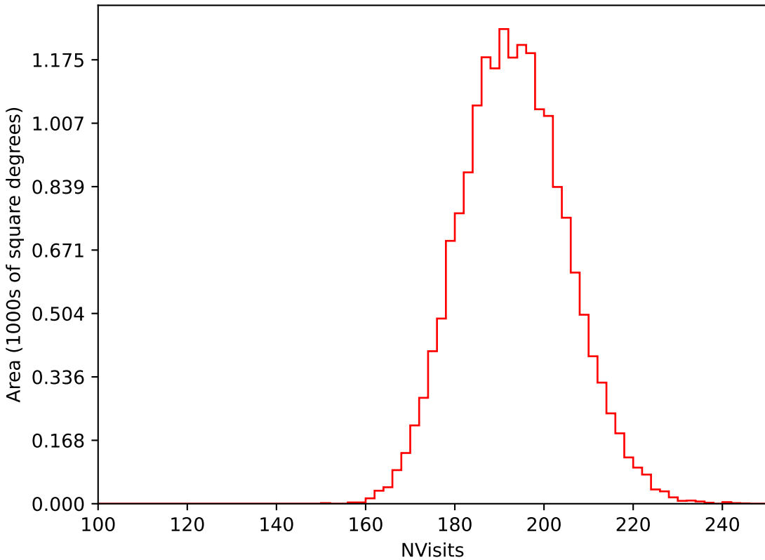
start_date_do-270v3.4_10yrs WFD i band: NVisits
