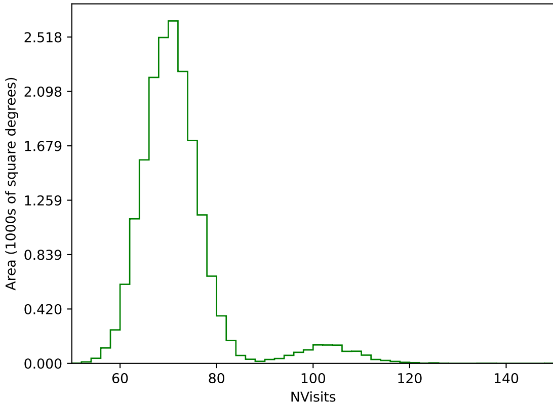
start_date_do-270v3.4_10yrs WFD g band: NVisits
