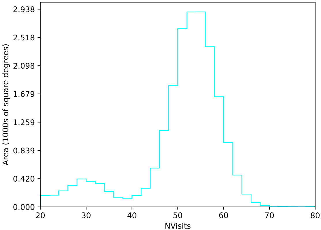
start_date_do-270v3.4_10yrs All sky u band: NVisits
