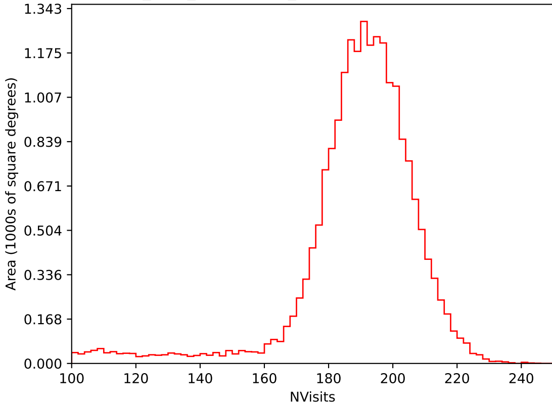
start_date_do-270v3.4_10yrs All sky i band: NVisits
